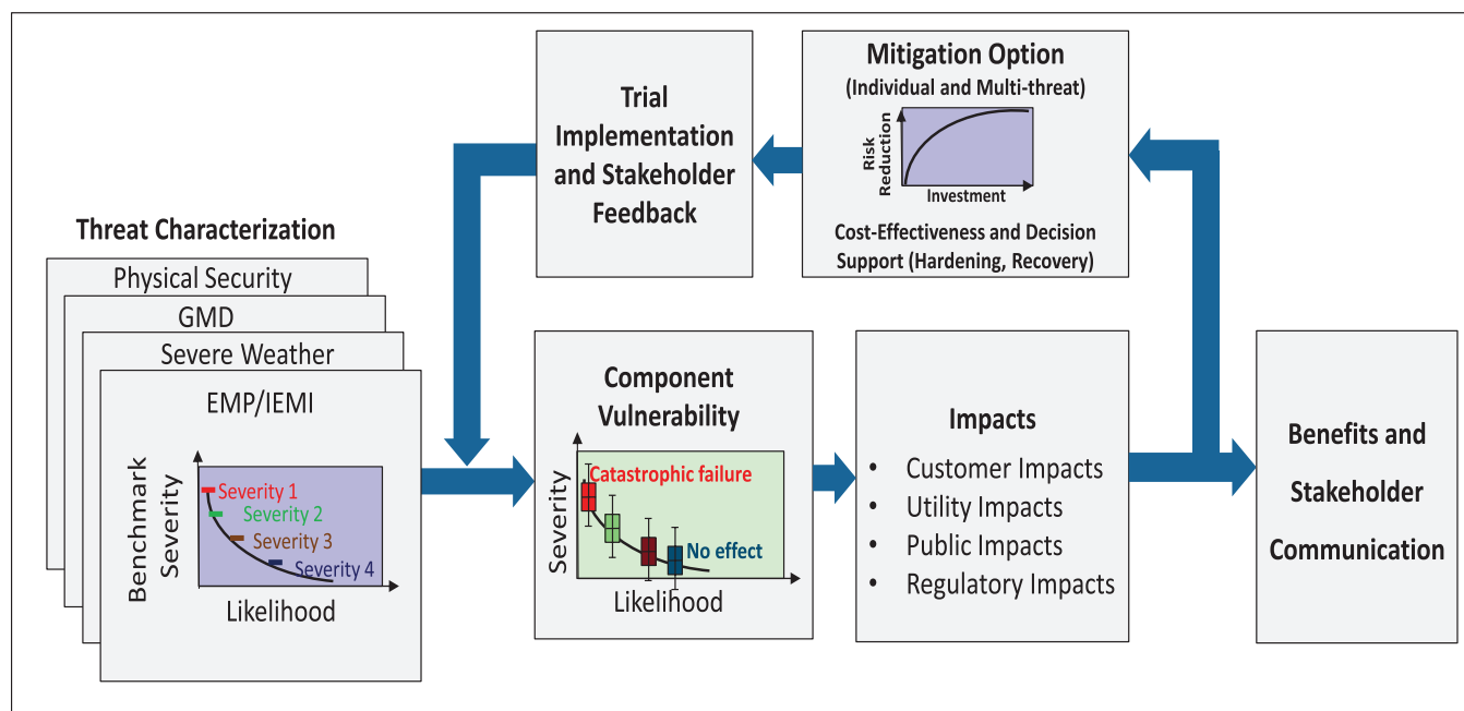
FIGURE 4.1 The process of considering and mitigating individual component vulnerability based on cost-performance optimization. NOTE: GMD, geomagnetic disturbance; EMP, electromagnetic pulse; IEMI, intentional electromagnetic interference.
