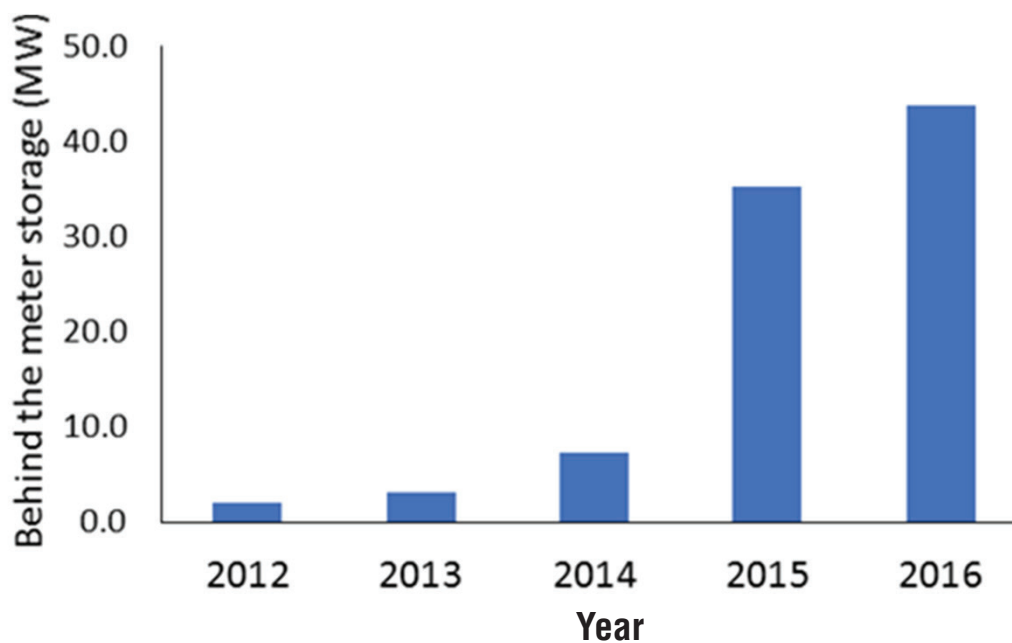
FIGURE 5.2 Installation of “behind the meter” battery storage systems. SOURCE: GTM Research/ESA (2016), “U.S. Energy Storage Monitor.”
